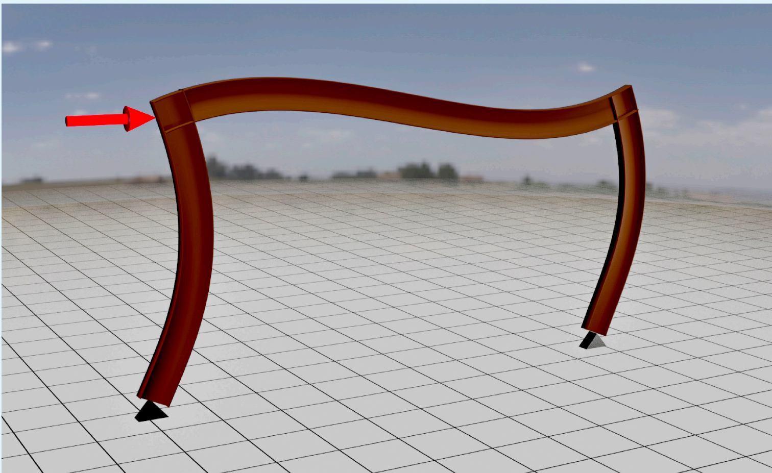
Lateral rigid frame with pinned base displacement
